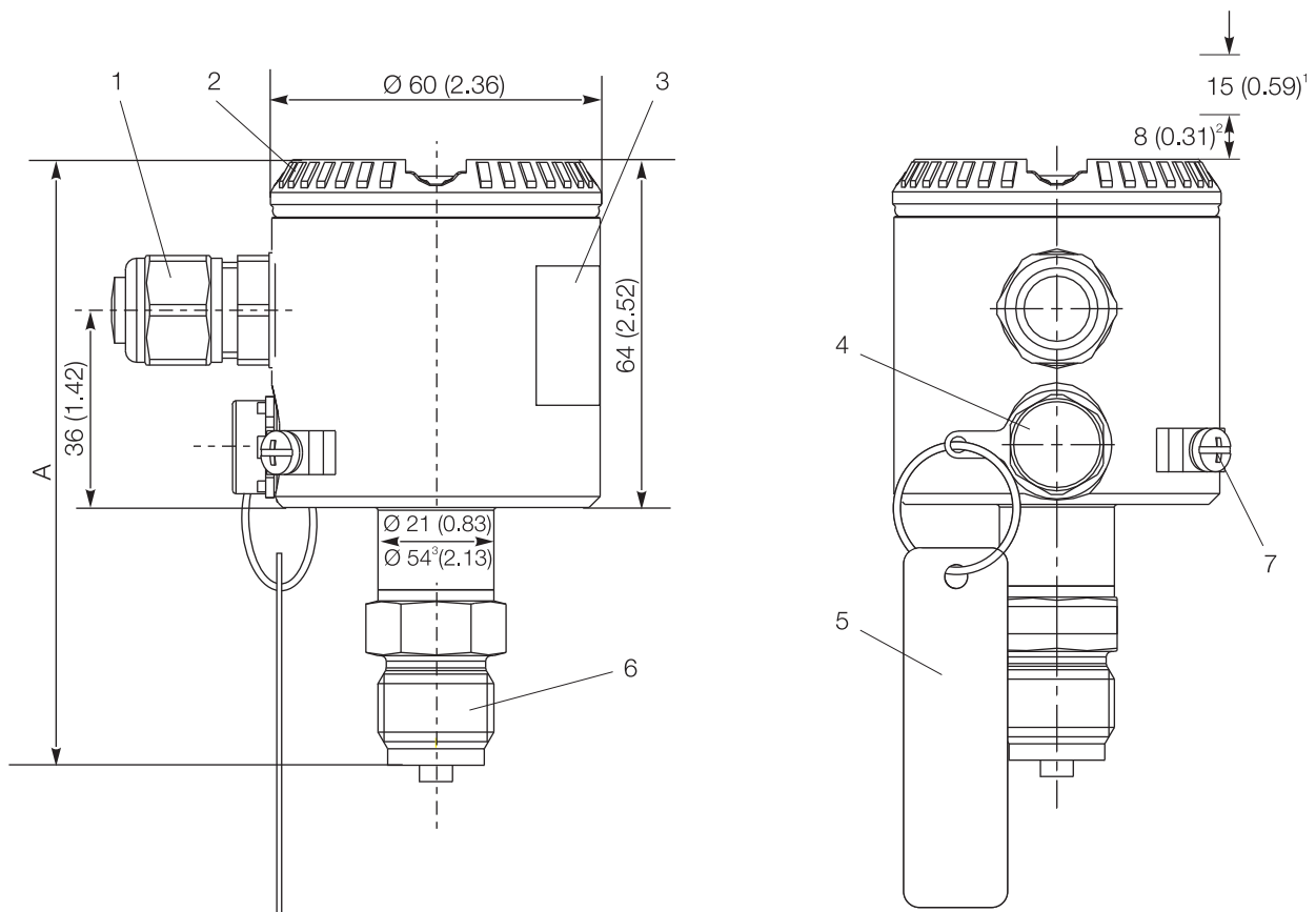
Fig. 1: Dimensions - Standard version
