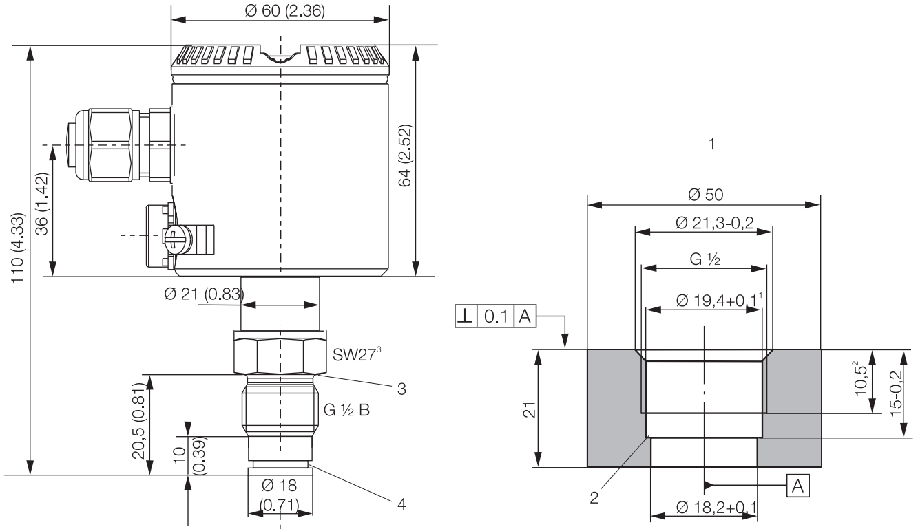
Fig. 3: Dimensions - With flush diaphragm
