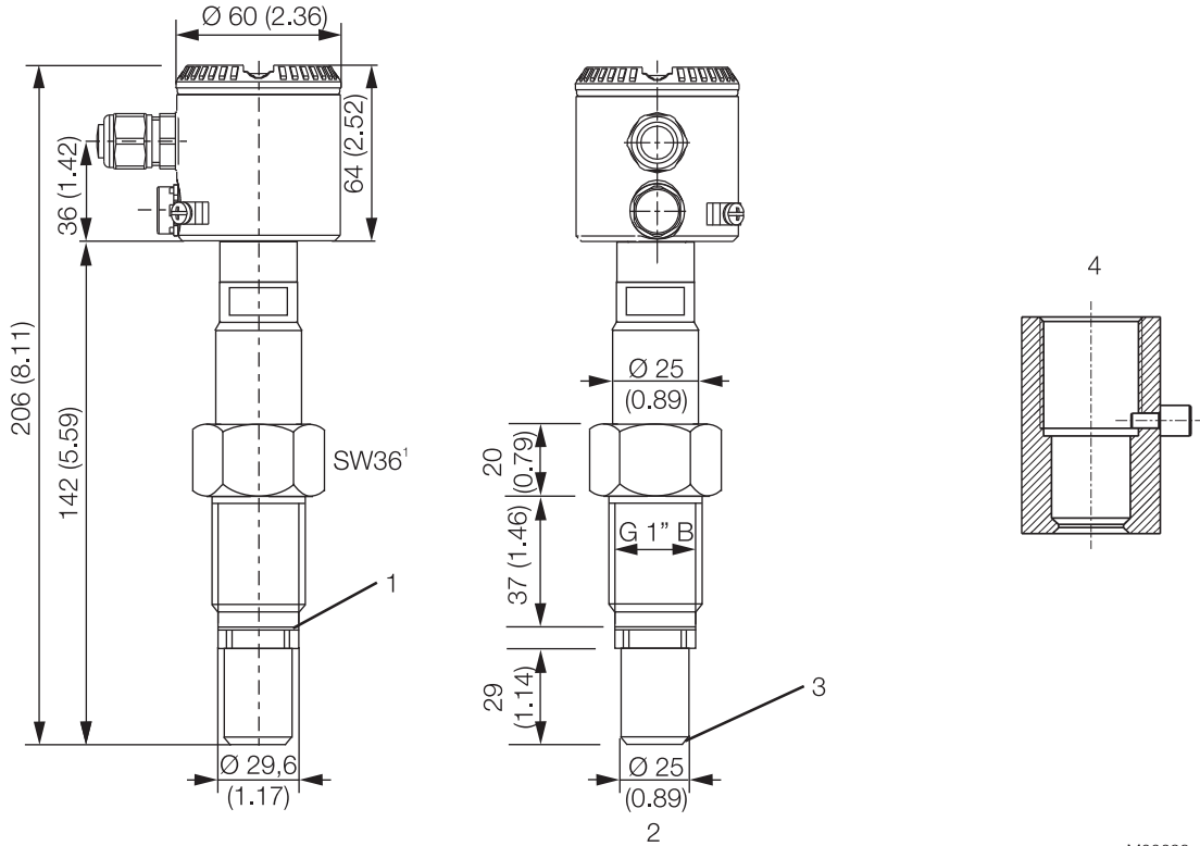
Fig. 4: Dimensions - With ball valve connection 1 Shim | 2 Diaphragm diameter: ~ 20 mm (0.79 inch) | 3 metal / metal conical seal, diaphragm is process-bonded | 4 Weld-in sleeve G 1", part no.: 789516
