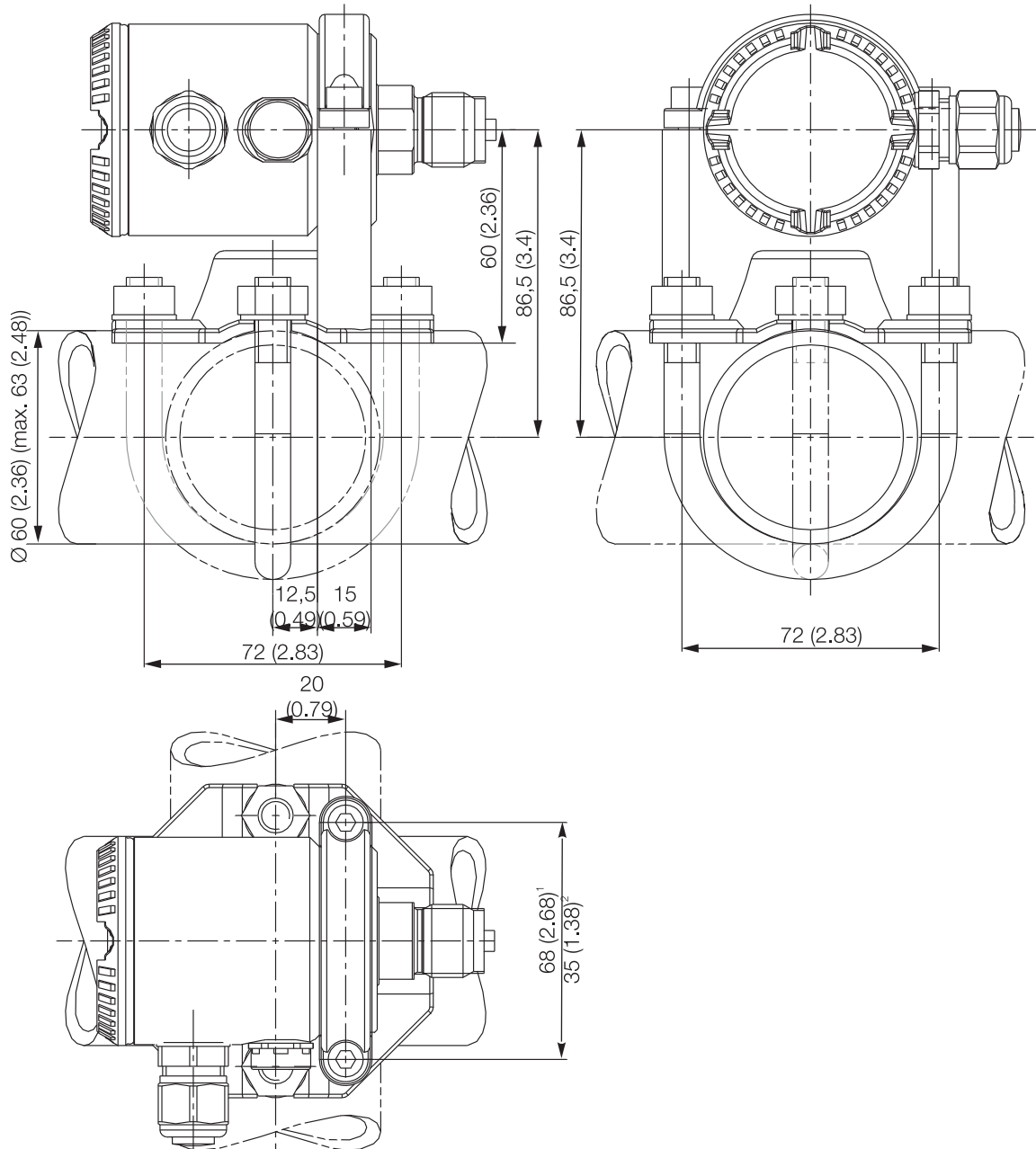
Fig. 5: Dimensions - Pipe / wall mounting
